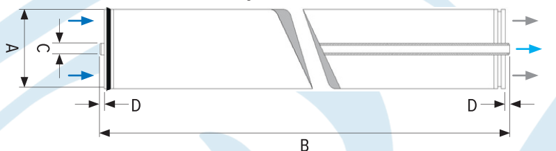
Figure 2: 8040 element
