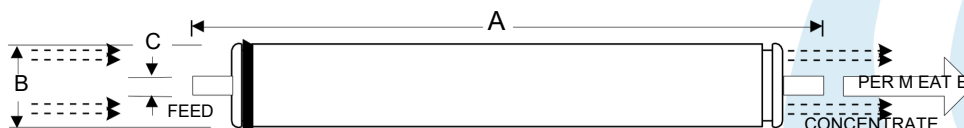
Element Details**
